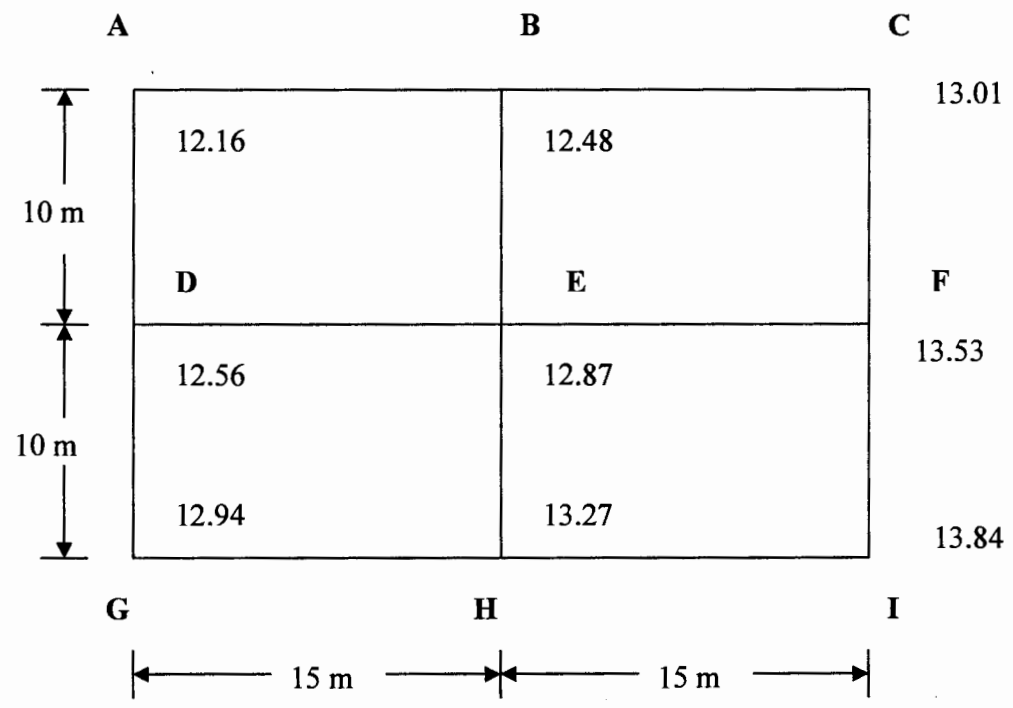
Figure 2. Reservoir spot heights for a levelling grid
